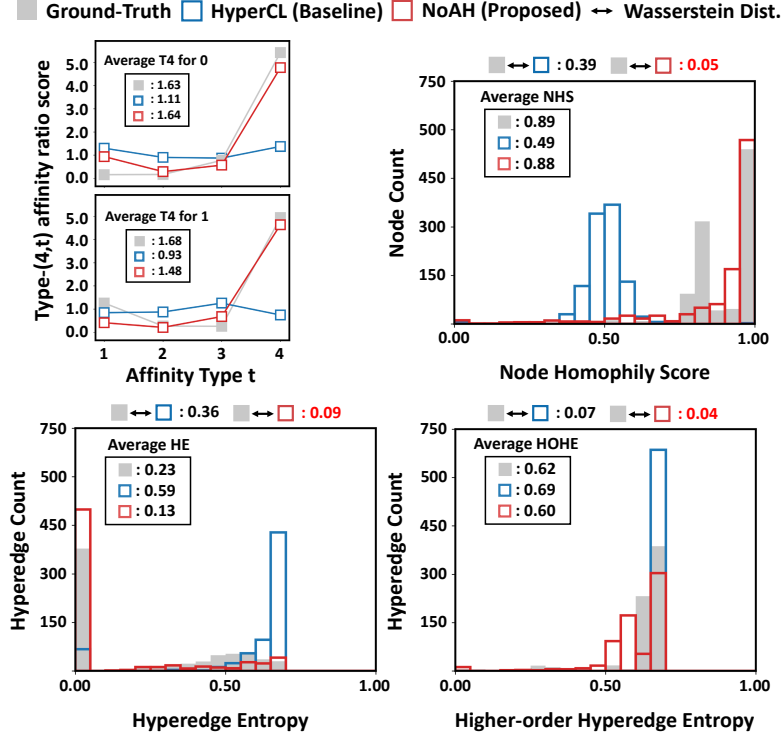
Fig. 1: Structure-attribute interplay with respect to the first node attribute in the Amazon Music dataset. Our proposed generative model, NoAH, fitted by its parameter learning algorithm NoAHFit, effectively captures the interplay between structure and node attributes, outperforming the baseline model (HyperCL). Refer to Section 3.2 for the definitions of the measures and to Section 7.3 for the interpretation of the results.
