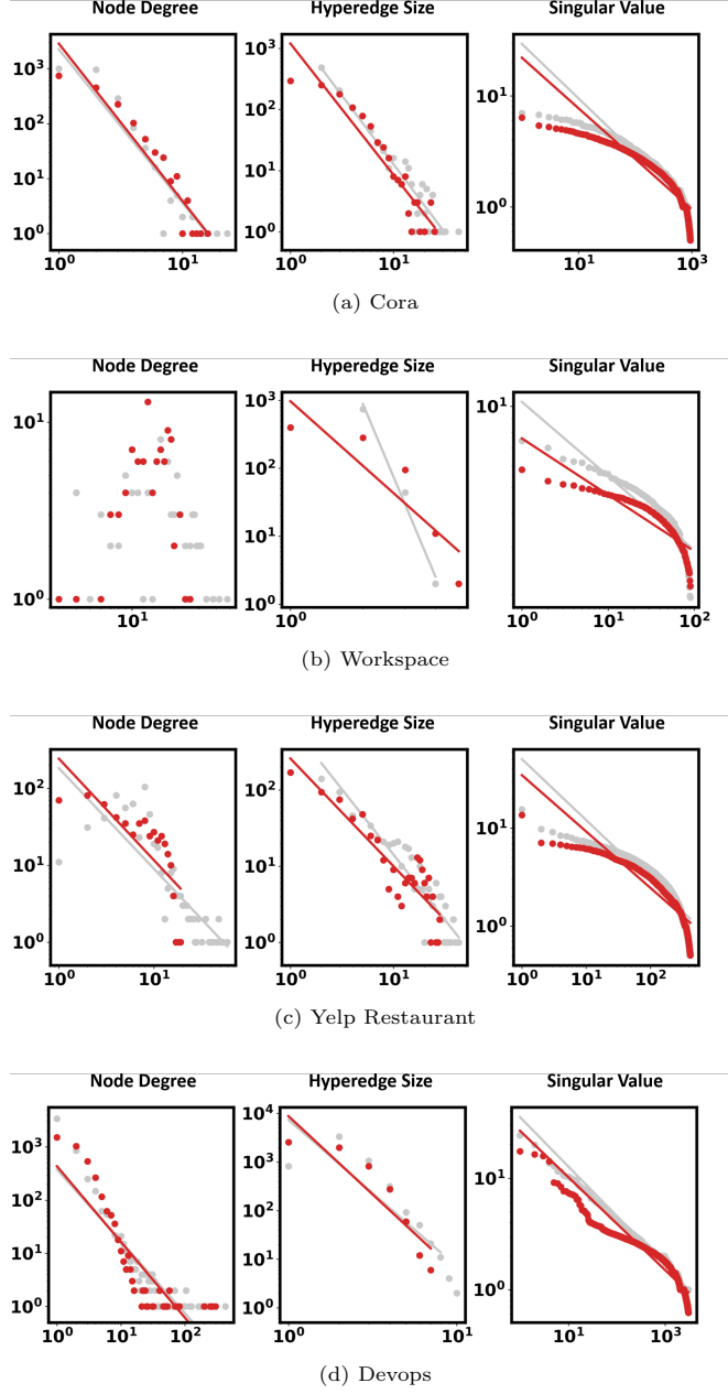
Fig. 8: Structural patterns of real-world hypergraphs (gray) and those generated by NOAH tuned by NOAHFIT (red). These results demonstrate that, despite its focus on structure–attribute interplay, NOAH also successfully reproduces purely structural patterns.
