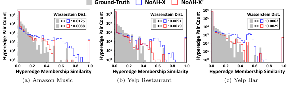
Fig. 6: Hyperedge diversity in the setting without pre-existing attributes. We report the distribution of pairwise similarity between (the node sets of) generated hyperedges in terms of Jaccard similarity. NOAH-X tends to yield more highly similar hyperedge pairs, whereas NOAH-X + more closely matches the ground-truth distribution by increasing diversity through hyperedge-wise attribute sampling.
