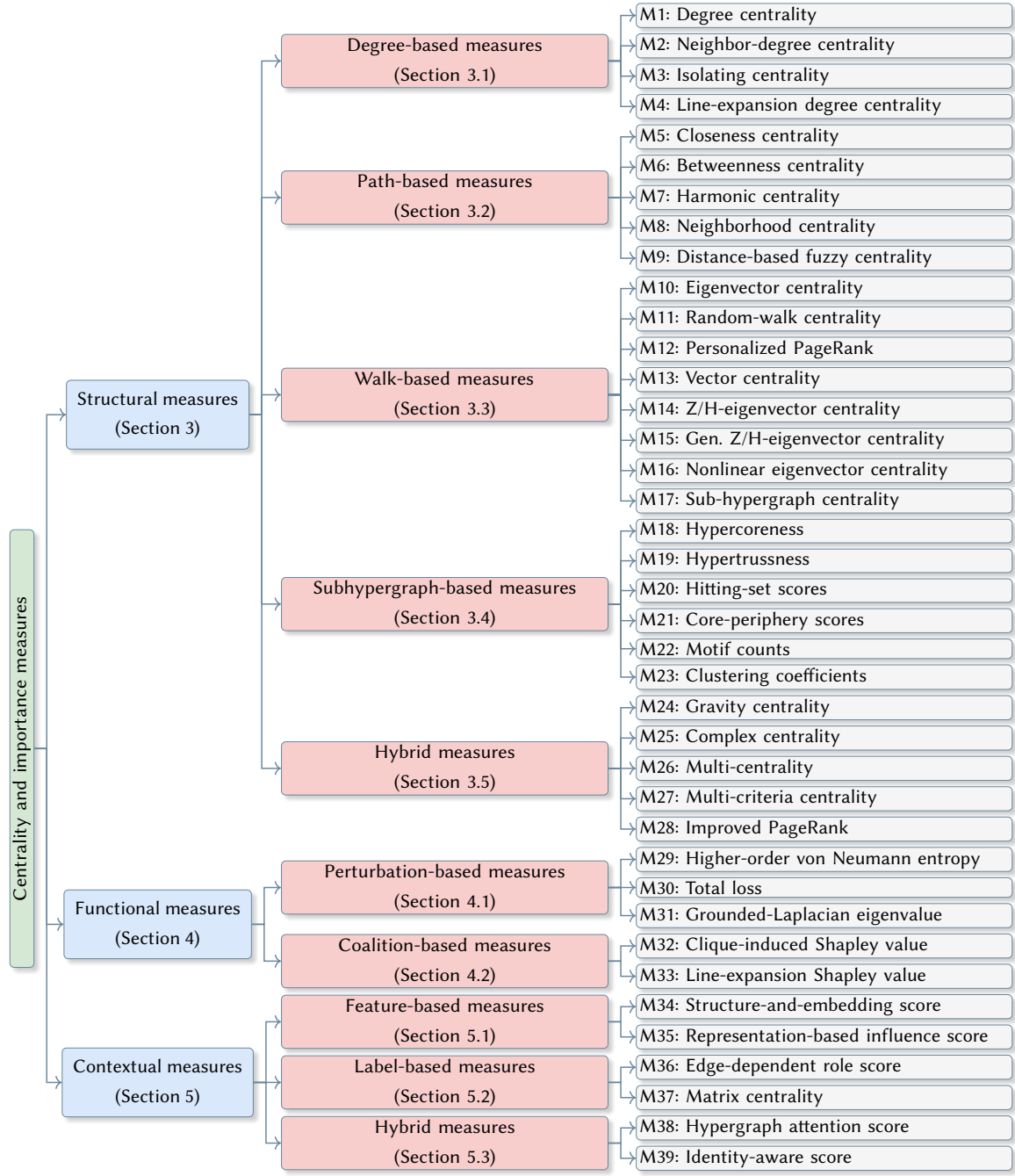
Fig. 2. Taxonomy of hypergraph centrality and importance measures. The framework distinguishes three major categories: structural measures, which rely on the combinatorial structure of the hypergraph; functional measures, which evaluate importance in terms of system behavior; and contextual measures, which integrate information beyond structure. Each category is further divided into sub-categories that capture specific methodological choices.
