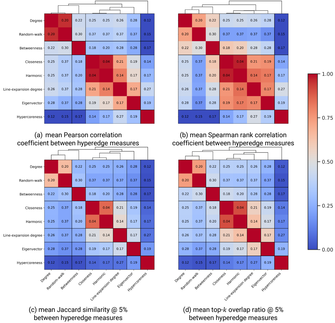
Fig. 4. Correlation between hyperedge centrality and importance measures in terms of (a) Pearson correlation coefficient, (b) Spearman rank correlation coefficient, (c) Jaccard similarity @ 5%, and (d) top- k overlap ratio @ 5%. The colormap indicates the average value of each measure across all datasets, and we annotate the standard deviation across datasets in each cell.
