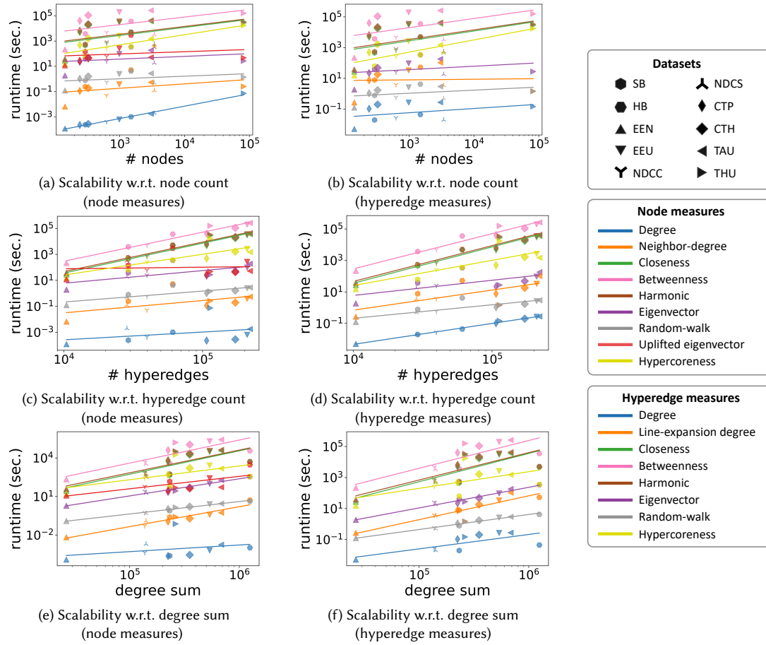
Fig. 5. Computation time of node and hyperedge measures with respect to different structural quantities on a log-log scale. Each subfigure reports the total computation time with respect to (a & b) the number of nodes, (c & d) the number of hyperedges, and (e & f) the total degree sum, for node and hyperedge measures, respectively.
