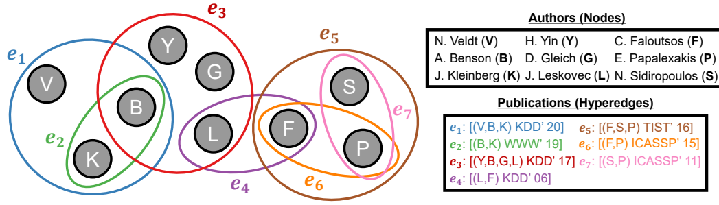
(a) Example hypergraph constructed from a co-authorship network. Nodes represent authors and hyperedges represent publications containing the corresponding sets of authors.
