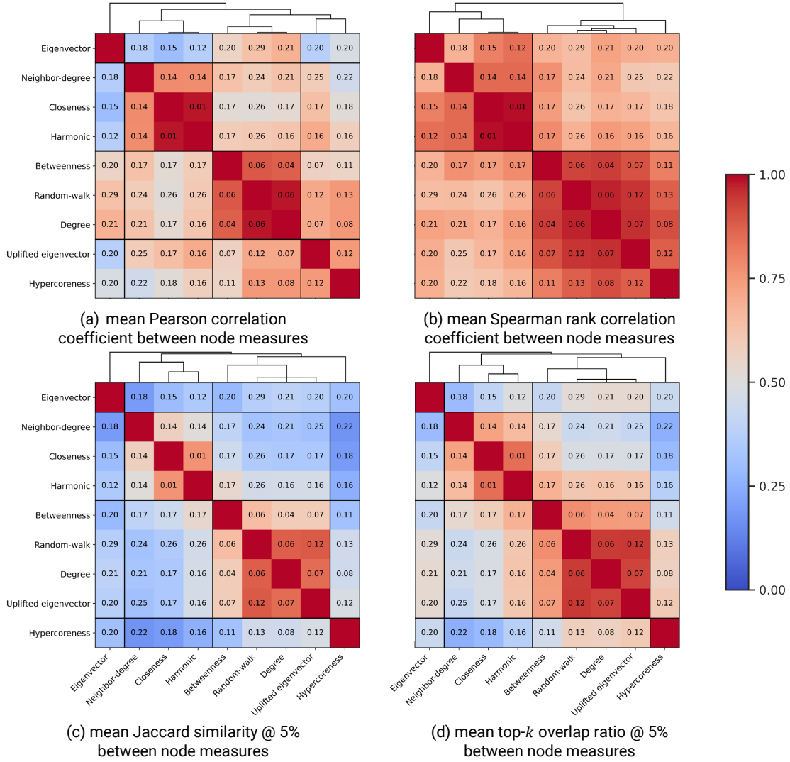
Fig. 3. Correlation between node centrality and importance measures in terms of (a) Pearson correlation coefficient, (b) Spearman rank correlation coefficient, (c) Jaccard similarity @ 5%, and (d) top-k overlap ratio @ 5%. The colormap indicates the average value of each measure across all datasets, and we annotate the standard deviation across datasets in each cell.
